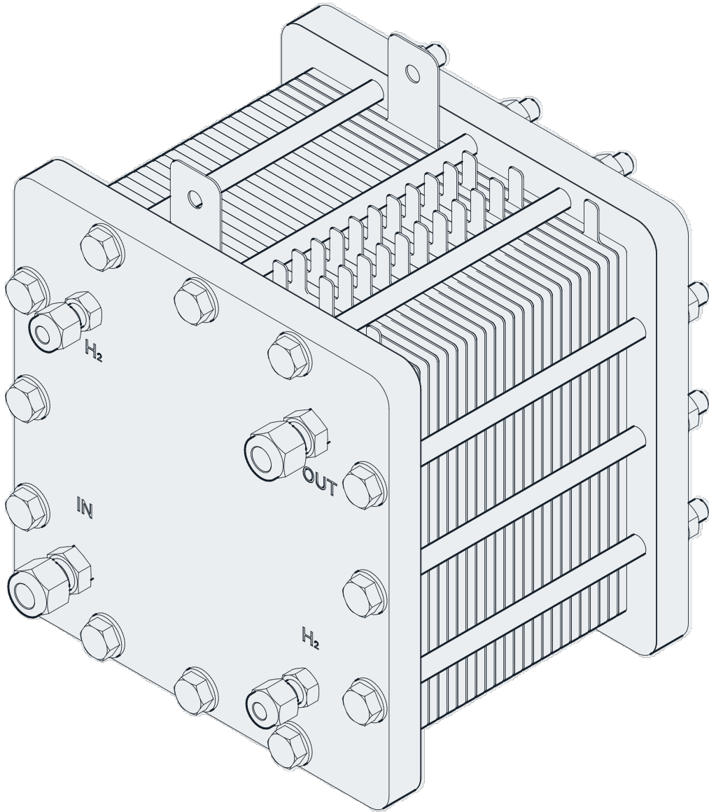
입체도 · ISOMETRIC (NTS)
