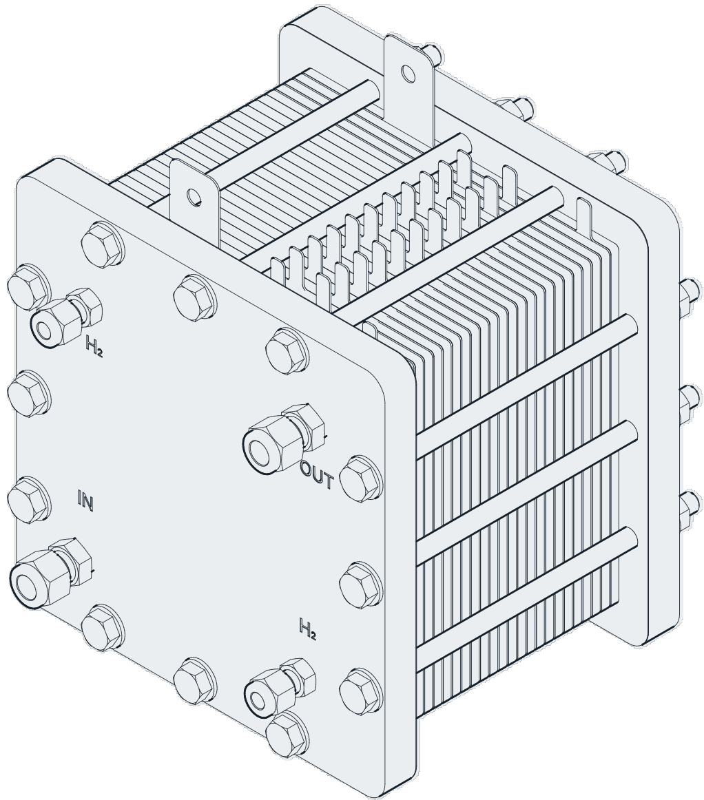
ISOMETRIC (NTS)
